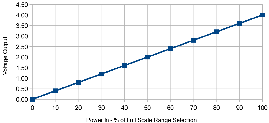
DPS-100D Voltage Output vs % Full Scale Range
